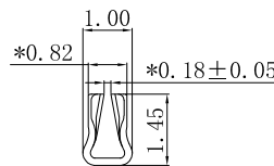
SEC:C-C
